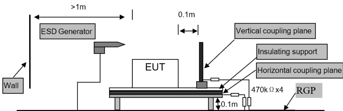
Floor-standing equipment
